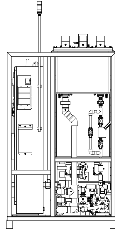
RIGHT VIEW
