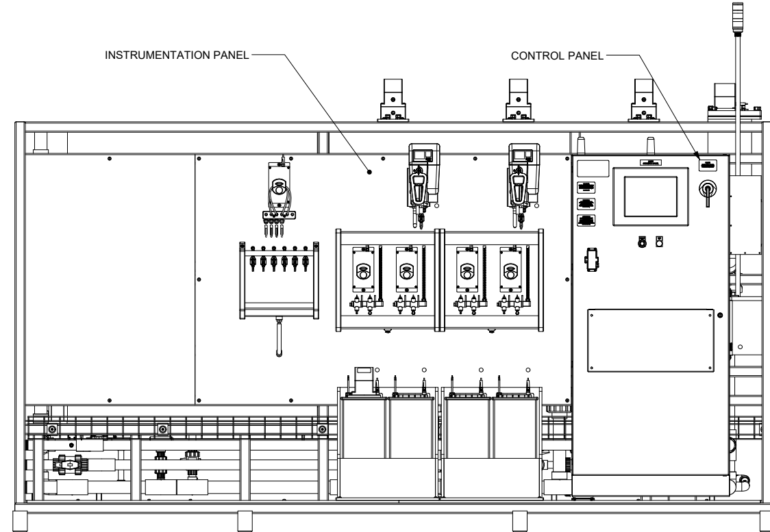
BACK VIEW
