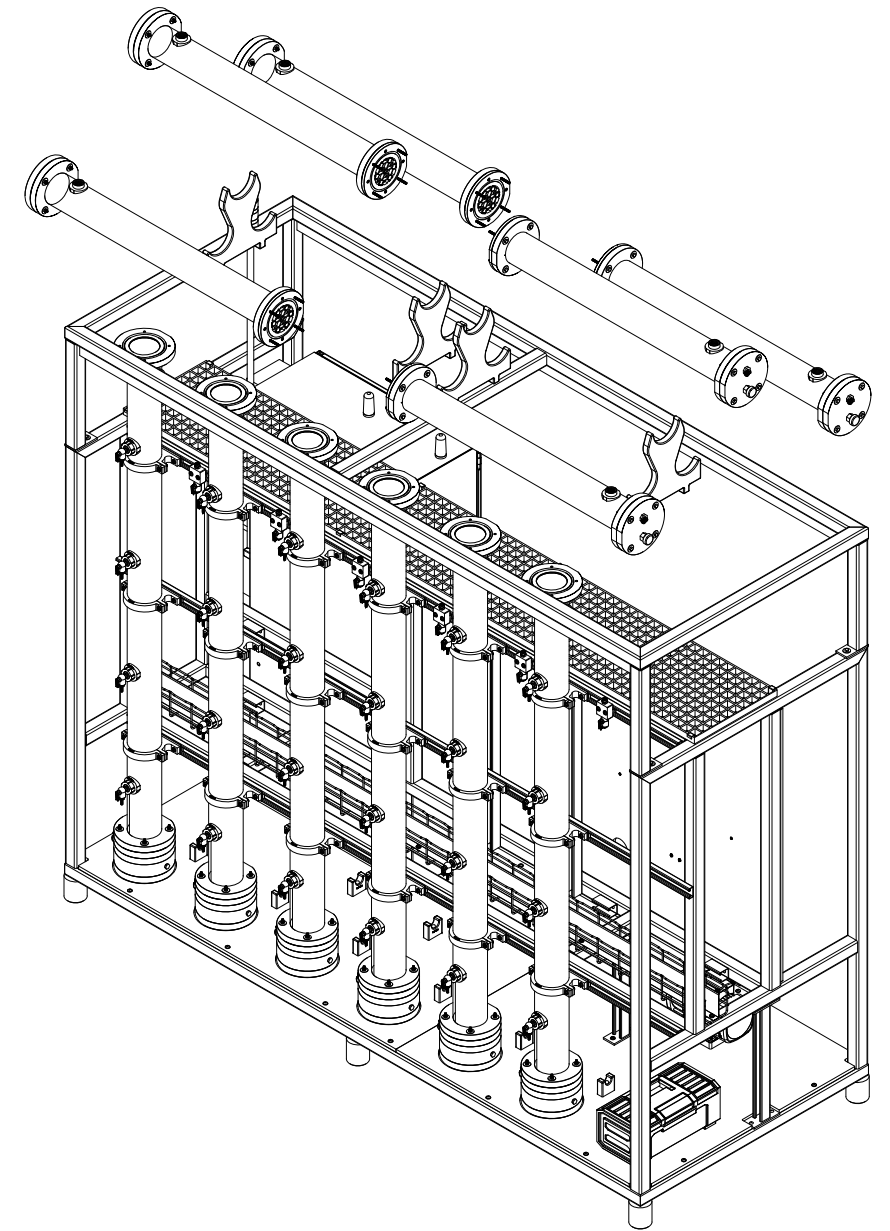
EXPLODED VIEW
